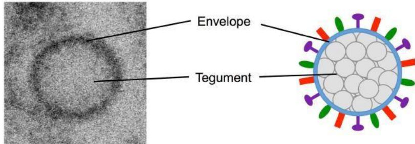
L-particle
